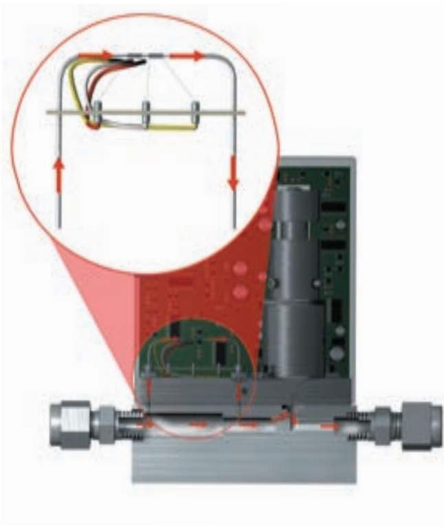
Figure 1. Cutaway of sensor technology.
