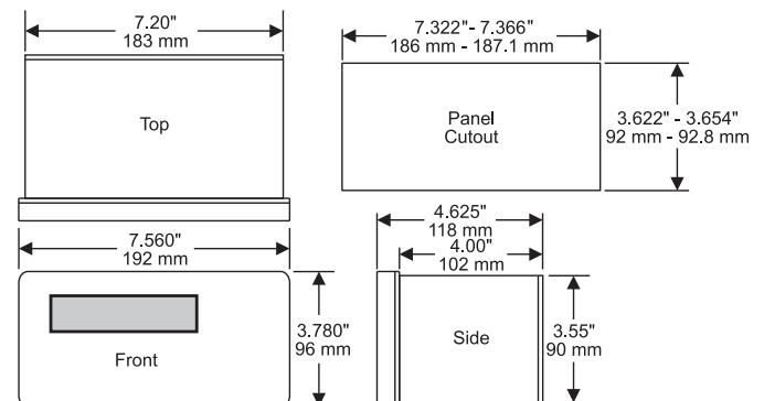
Panel Mount
