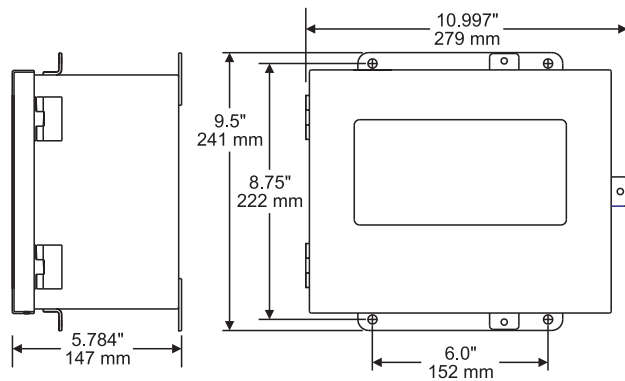
Wall Mount
